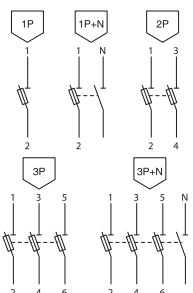
20SC400031 F0202
